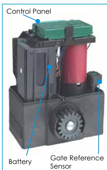
D5 Control Panel
